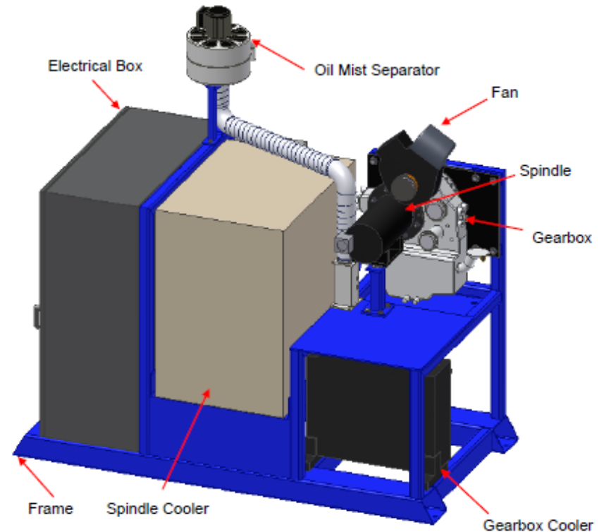
Typical Cooling Fan Test Stand components
