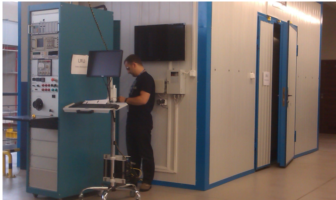
Cooling Fan Test Stand under test (control console outside the sound attenuated enclosure containing the unit under test)
